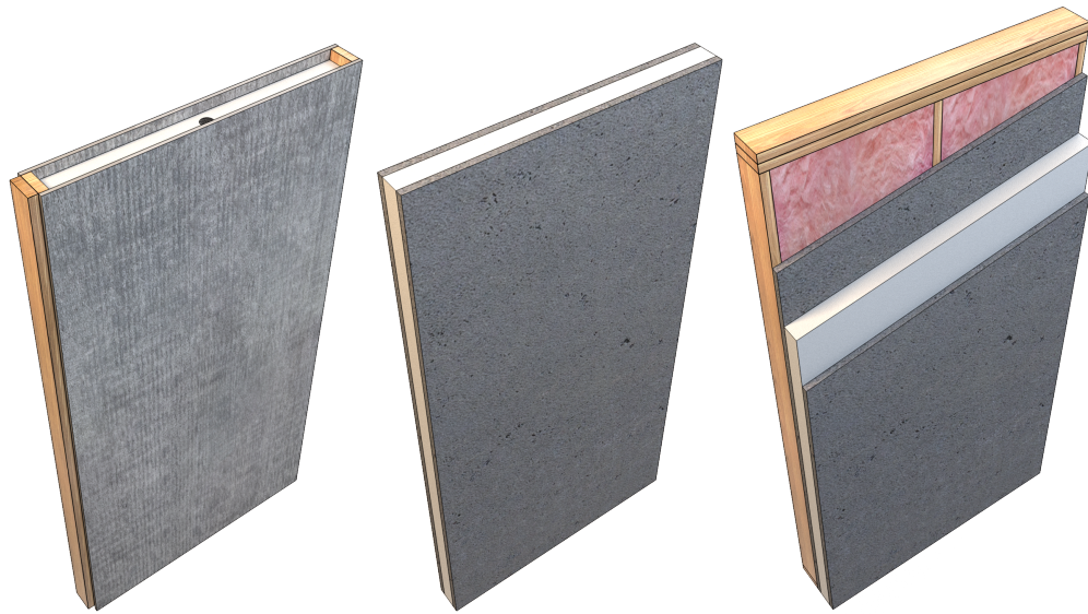
Double Wall Concrete Panel & Stick Frame 4' x 8'
